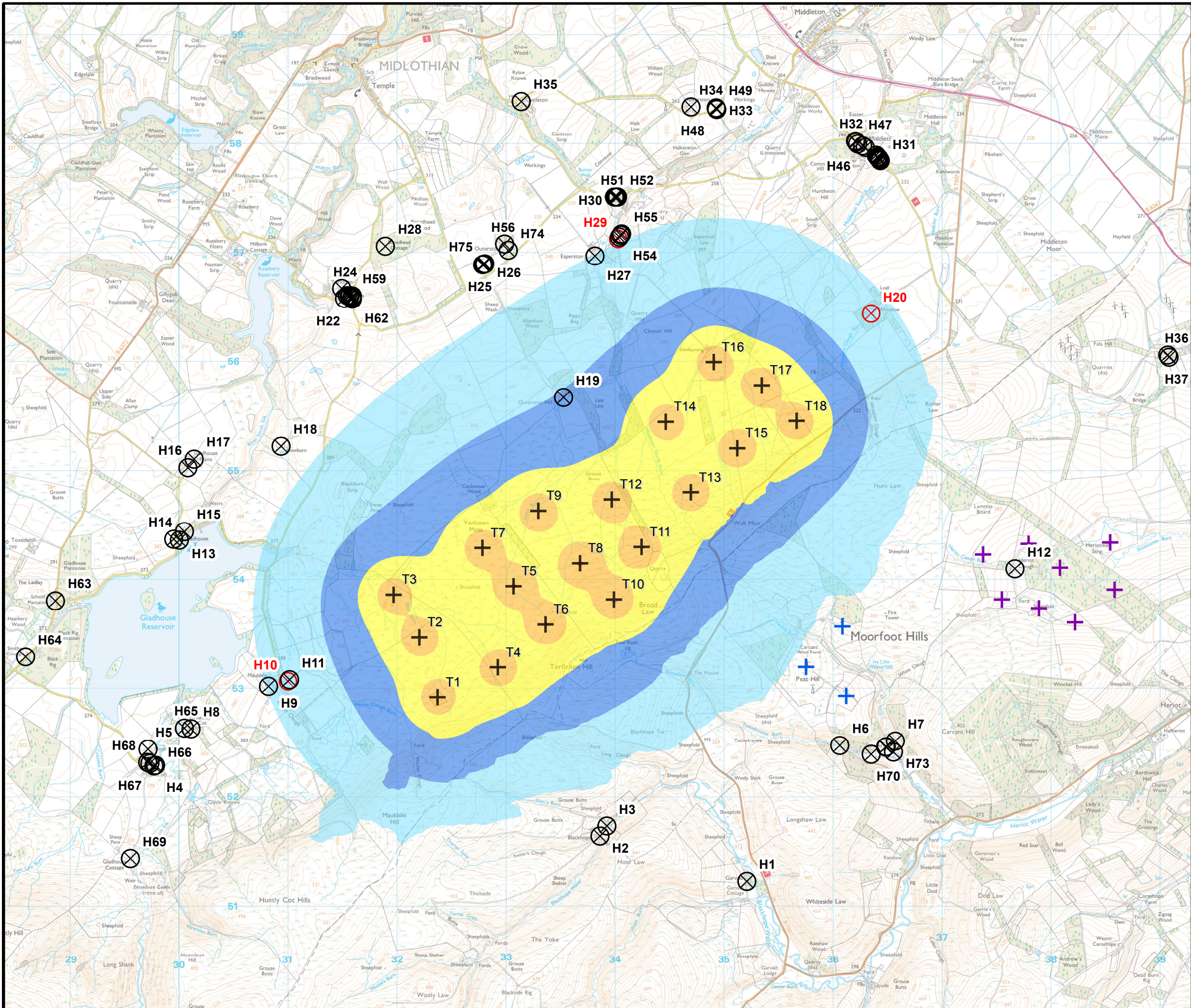
FIGURE 12.1 NOISE CONTOUR PLOT
